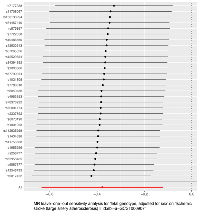
Fig. S2. Leave-one-out analysis for the associations of placental weight with ischemic stroke (large artery atherosclerosis)
