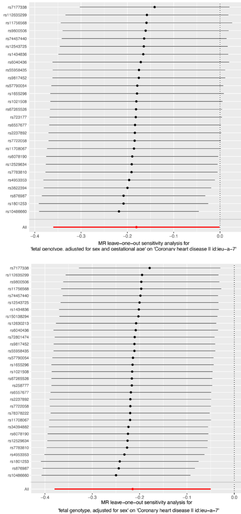
Fig. S1. Leave-one-out analysis for the associations of placental weight with coronary heart disease
