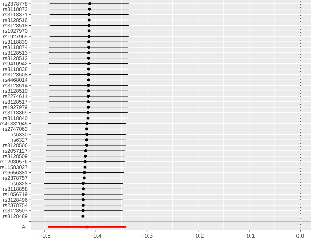
Supplementary Figure S2. Leave-one-out analysis of the causal effect of 18 inflammatory proteins on Colorectal cancer
