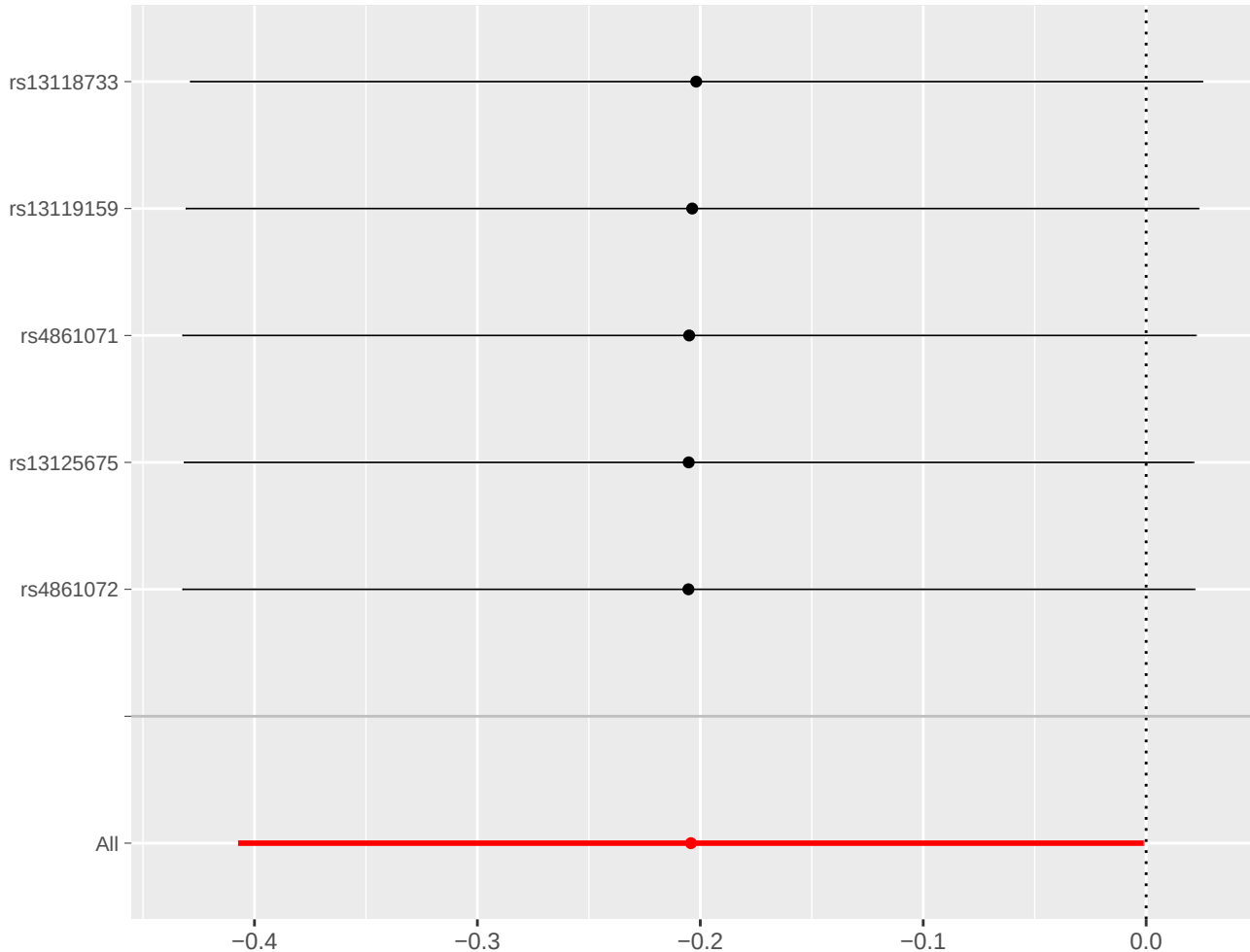
MR leave-one-out sensitivity analysis for 'Interleukin-13 levels' on 'Colorectal cancer'
