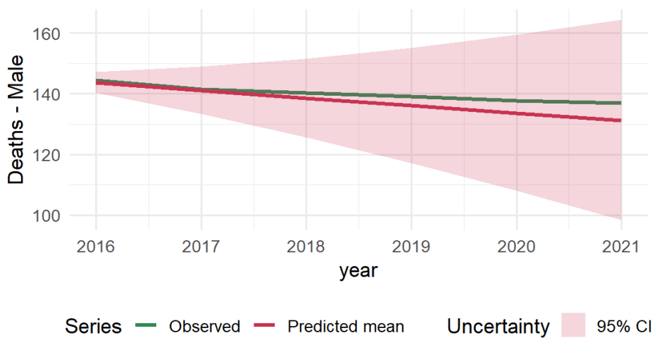
Supplementary Figure S3. Back validation of BAPC predictions
