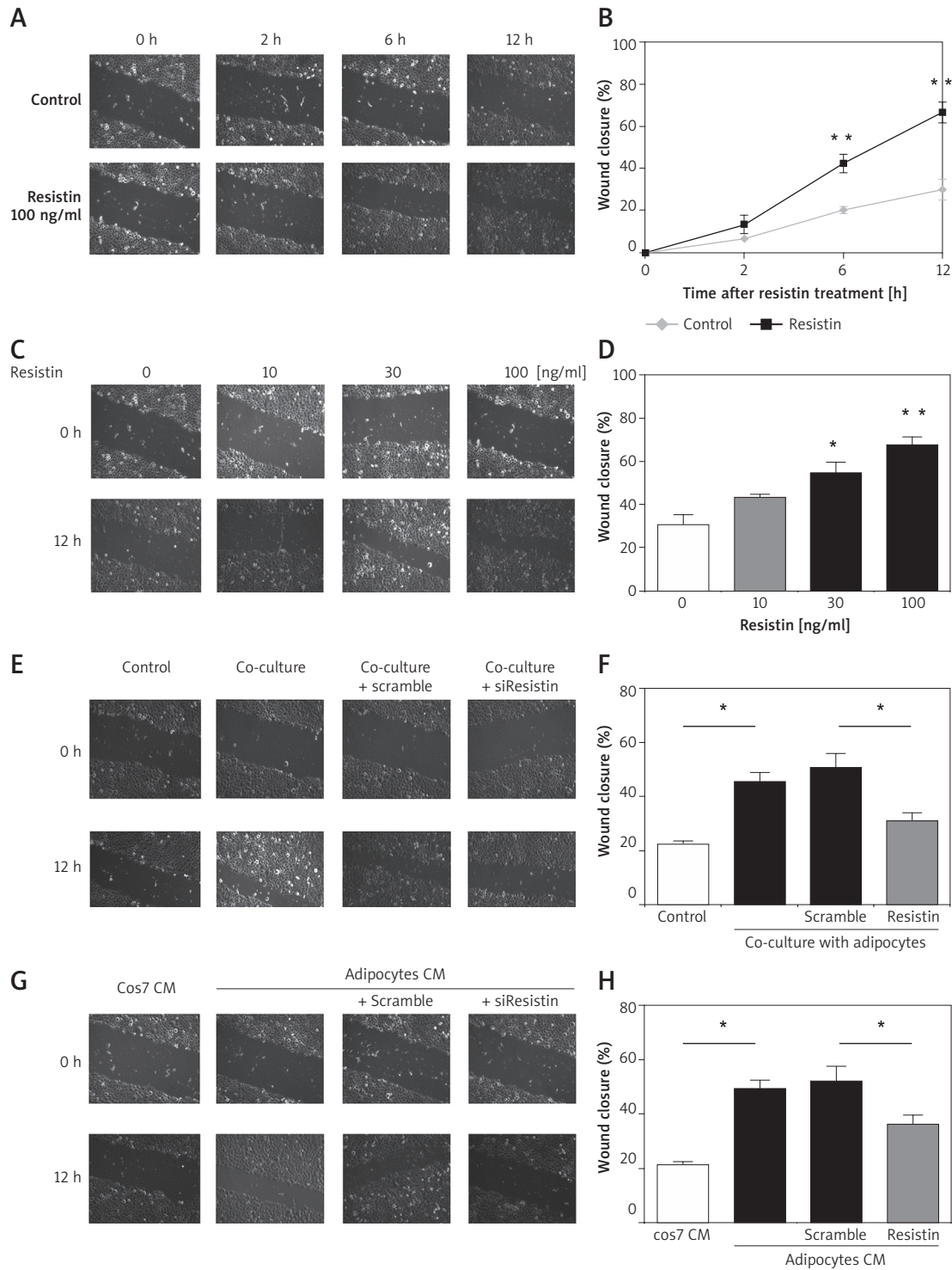
Figure 3. Effect of resistin on HO-8910 cell migration and interference of siRNA in the resistin-mediated effect on co-culture migration. A, B – Time course of the effects of treatment with 100 ng/ml resistin on the wound-healing rates of HO-8910 cells. C, D – Dose-response effect of 12 h treatment with resistin on the wound-healing rate of HO-8910 cells. E, F – The wound-healing rate with resistin compared to that with the knockout of resistin in the co-culture system. Co-cultured cells were incubated with 100 ng/ml resistin for 12 h. G, H – Cos-7 cells were used as negative controls; adipocyte-conditioned media significantly promoted the wound-healing rate of HO-8910 cells. The wound-healing rate was attenuated by the knockout of resistin in a co-culture system
