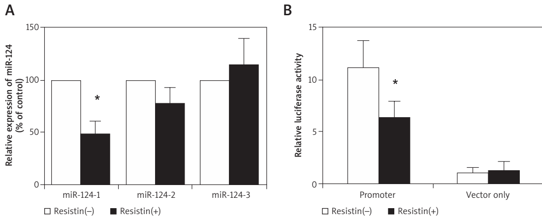
Figure 4. Effect of miR-124 on resistin expression and HO-8910 cell migration. A – The effect of resistin on miR-124 expression. HO-8910 cells were pretreated with or without resistin, then incubated with 100 ng/ml resistin for 24 h. miR-124-1 expression was attenuated by resistin in HO-8910 cells. MiR-124-2 and miR-124-3 expression was not affected by resistin. B – Effects of miR-124 on resistin promoter activity in HO-8910 cells
