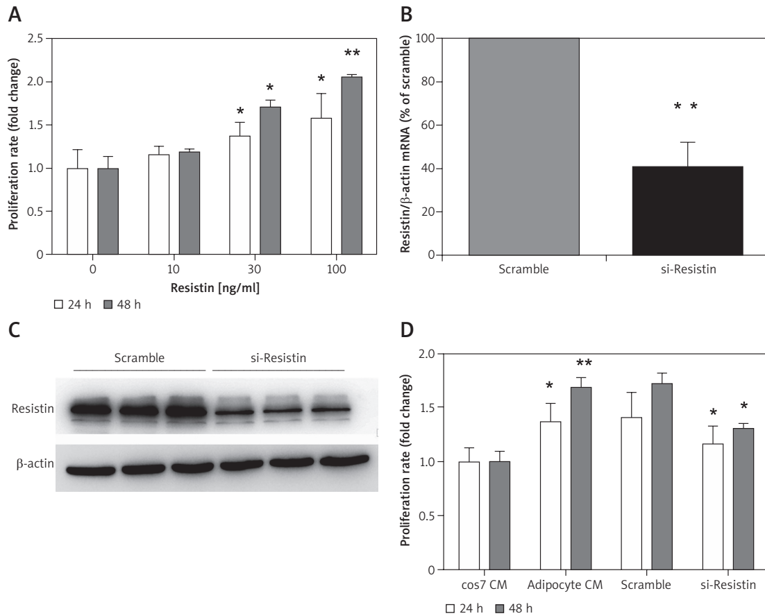
Figure 1. Effect of resistin on the proliferation of ovarian epithelial carcinoma HO-8910 cells. A – Time course of effects of treatment with 30–100 ng/ml resistin on the proliferation rate of HO-8910 cells. Dose-response effect of resistin on the proliferation of HO-8910 cells at 48 h after treatment. B – Small interfering RNA (siRNA) interferes with resistin expression at the mRNA and protein levels. As shown by real-time quantitative PCR, mRNA expression of resistin was decreased to 38% by resistin knockdown in adipose cells. C – Western blotting showed that the protein expression of resistin was reduced to 32% by the knockdown of resistin in adipose cells. D – siRNA interferes with adipocyte expression of resistin and decreases the proliferative effects of adipocyte-conditioned media. Cos-7 cells were used as negative controls. Adipocyte-conditioned media significantly promoted the proliferation of HO-8910 cells. Knockdown of resistin expression during adipocyte culture attenuated proliferation-inducing effects of adipocyte-conditioned media
