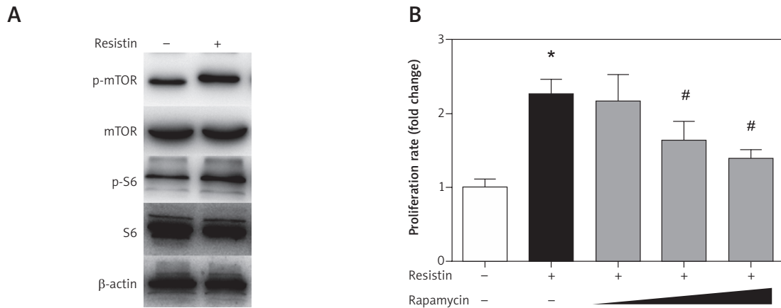
Figure 2. Involvement of mTOR (mechanistic target of rapamycin) signaling pathway in resistin-mediated induction of HO-8910 proliferation. A – Stimulation with resistin significantly elevated the phosphorylation of mTOR and S6 in HO-8910 cells. B – The mTOR inhibitor rapamycin significantly inhibited proliferation of HO-8910 cells that were pretreated with resistin
