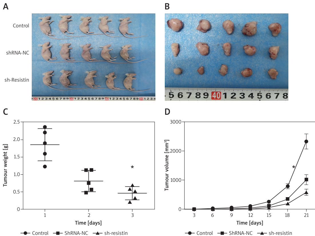
Figure 5. In vivo tumor xenograft study to elucidate the role of resistin. A, B – Nude mice from each group that showed tumor growth following the transplantation of control, shRNA-NC-transfected, and sh-resistin-transfected HO-8910 cells. C, D – Tumor volume was calculated every 3 days after injection, and the tumors were excised and weighed after 21 days (* p < 0.05 )
