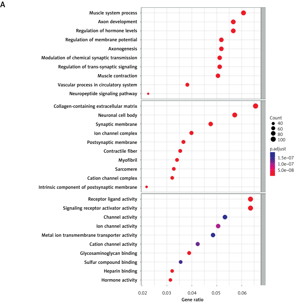
Figure 5. Gene Oncology (GO) and Kyoto Encyclopedia of Genes and Genomes (KEGG) enrichment analyses of high- and low-risk groups. A – Bubble map of GO and KEGG enrichment analyses
