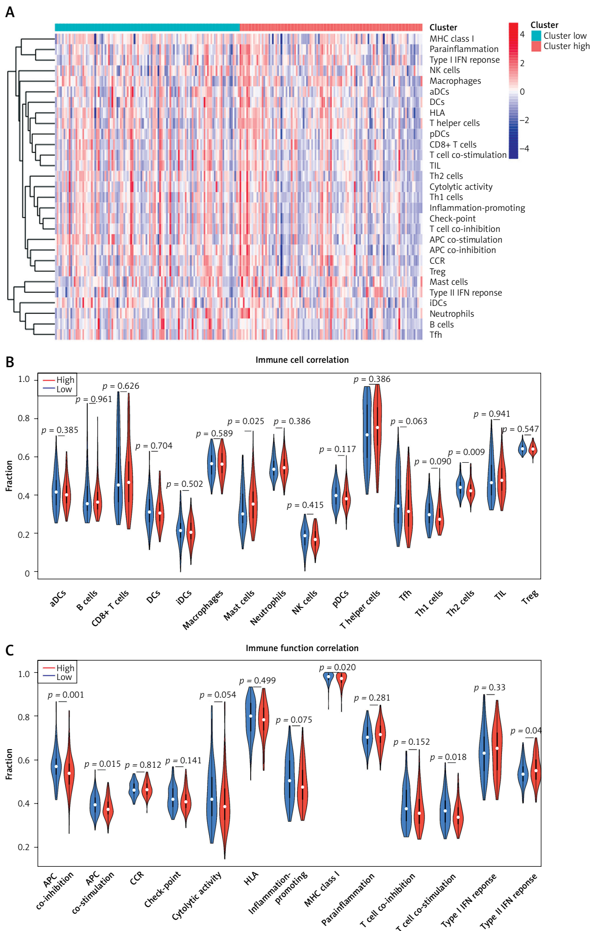
Figure 6. Single sample Gene Set Enrichment Analysis (ssGSEA) of high- and low-risk groups. A – Heat map depicts the expression of 29 immune cell gene sets in high- and low-risk groups. B – Violin plot of immune cell fraction differences in high- and low-risk groups. C – Violin plot of immunocompetence-related gene differences in high- and low-risk groups
