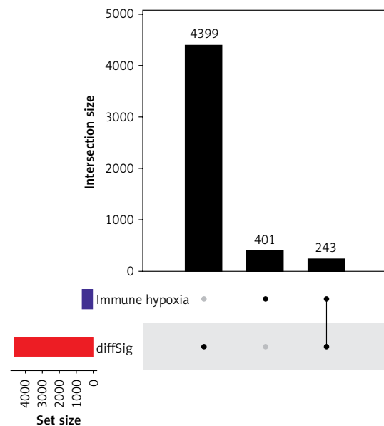
Figure 1. UpSet plot of the screening of hypoxia- and immune-related prognostic genes in STAD patients
