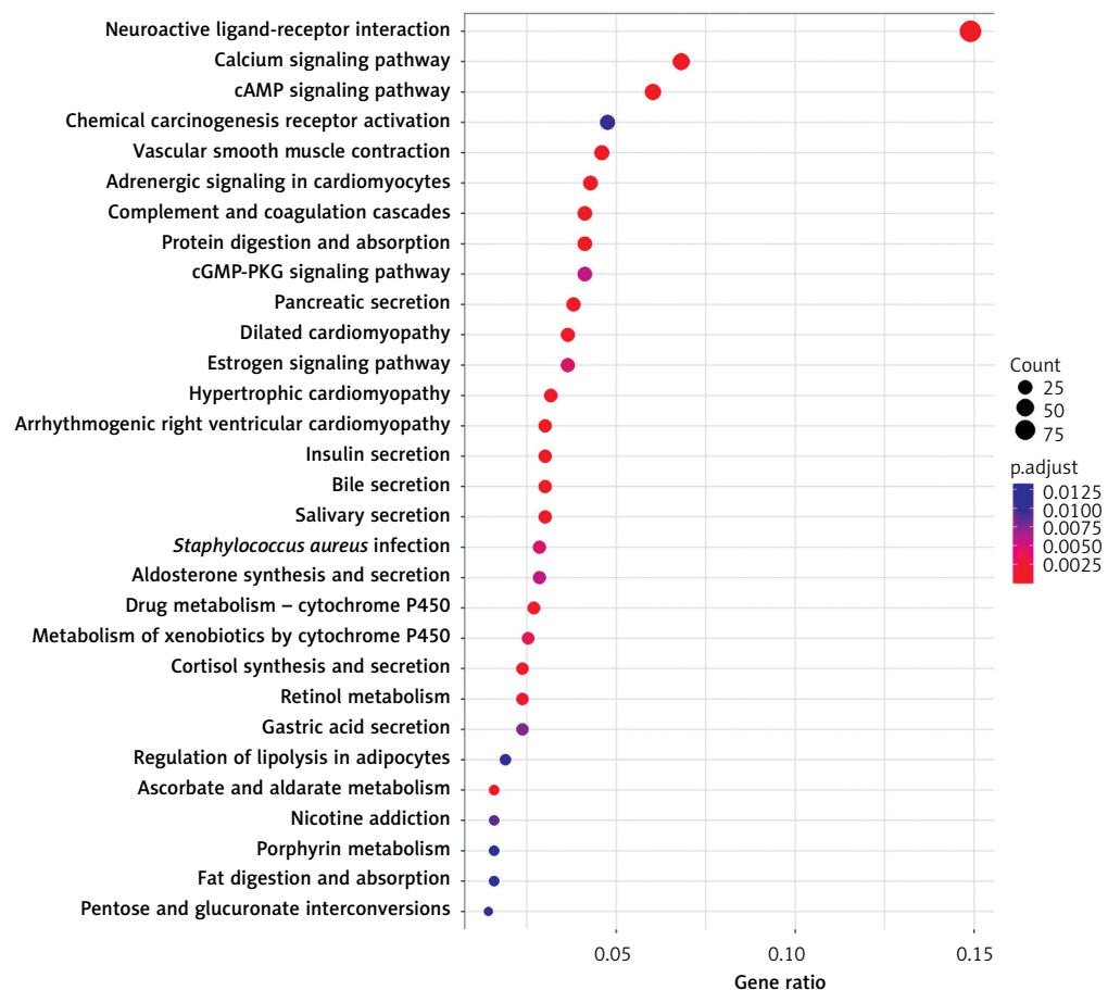
Figure 5. Cont. B – Bubble map of GO and KEGG enrichment analyses
