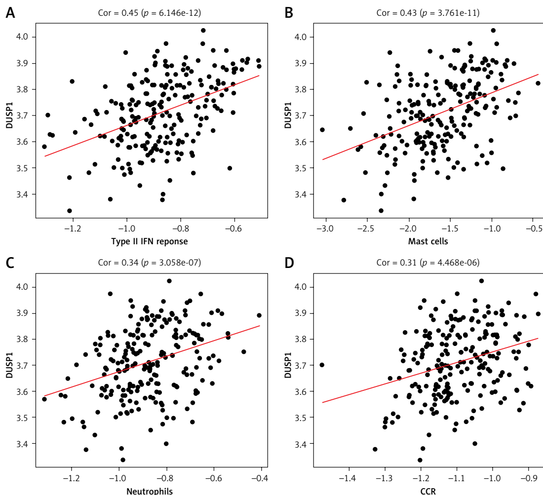
Figure 7. Correlation analysis of DUSP1 with immune-related cell and function scores. A – type II INF response; B – mast cell; C – neutrophils; D – CCR
