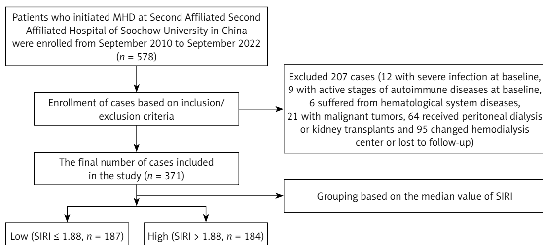
Figure 1. Flowchart of sample collection
