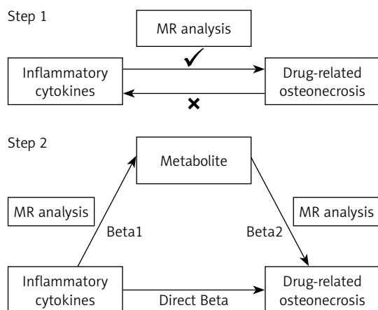
Figure 1. Flowchart of the MR analysis process
