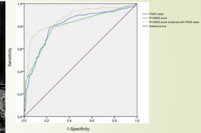
ROC curve analysis showed combination of PI-RADS score and PSAD had higher diagnostic performance compared with PI-RADS score or PSAD alone
