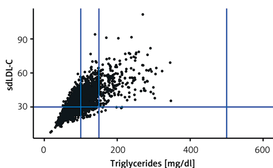
Figure 2. Relationship between serum small dense LDL cholesterol (sdLDL-C) and triglyceride levels. Serum sdLDL-C above 30 mg/dl was observed in borderline and moderate hypertriglyceridemia according to the EAS [3]
