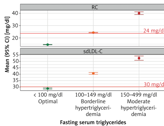
Figure 1. Mean (95% CI) serum remnant cholesterol (RC) and small dense LDL cholesterol (sdLDL-C) across triglyceride level intervals according to the EAS [3]
