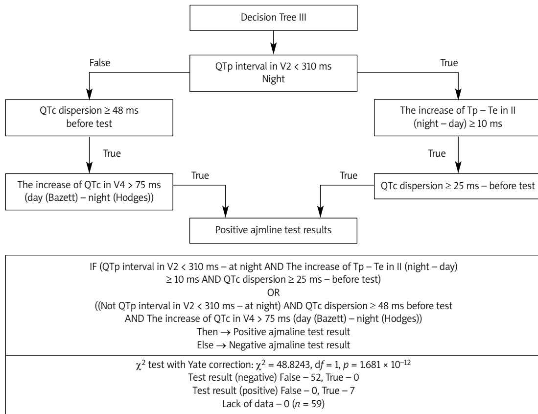
Figure 4. Decision Tree III
