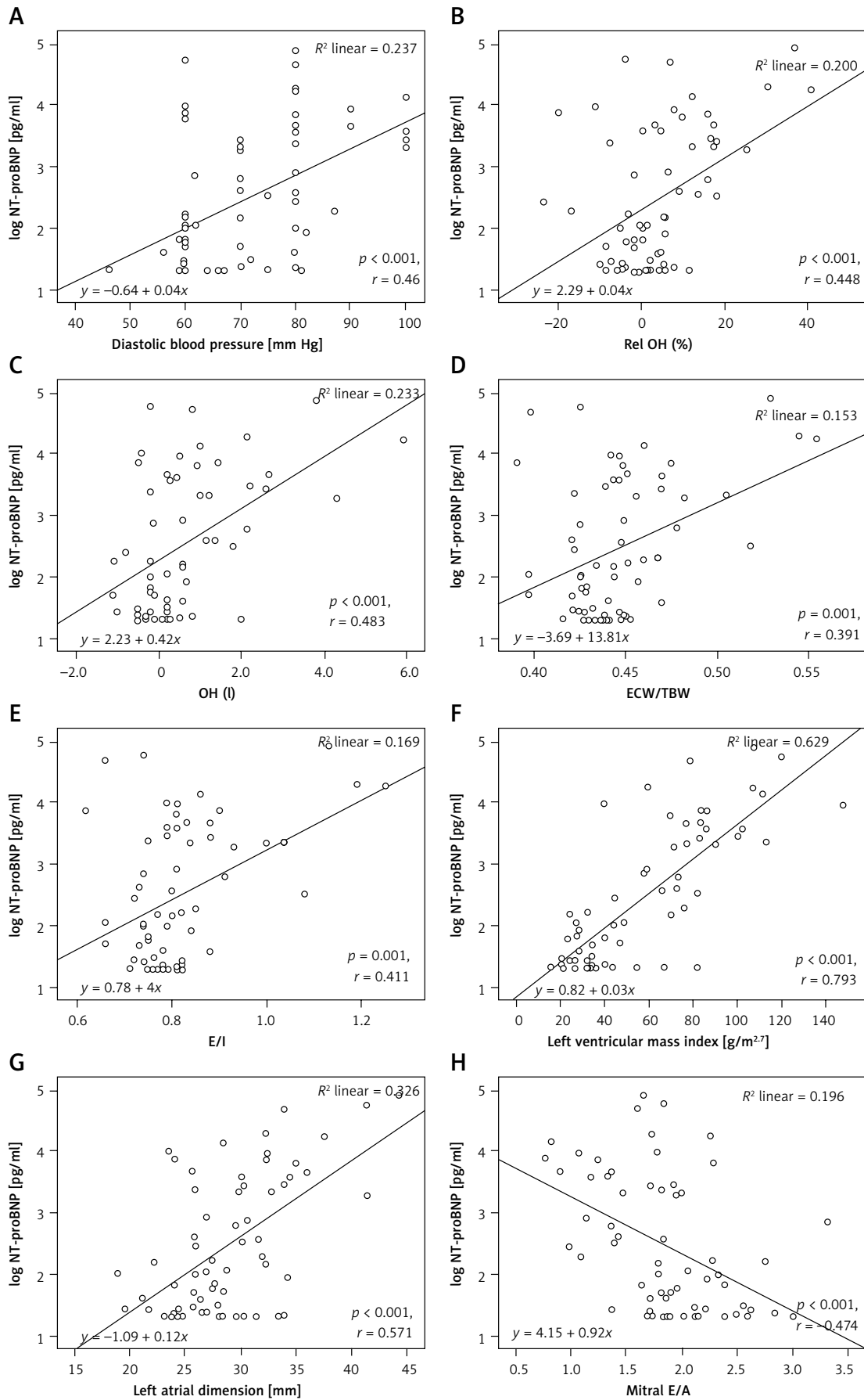
Figure 3. Correlation of log NT-proBNP level with diastolic blood pressure (A), Rel OH (B), OH (C), ECW/TBW (D), E/I (E), LVMI (F), LAD (G), mitral E/A (H)
