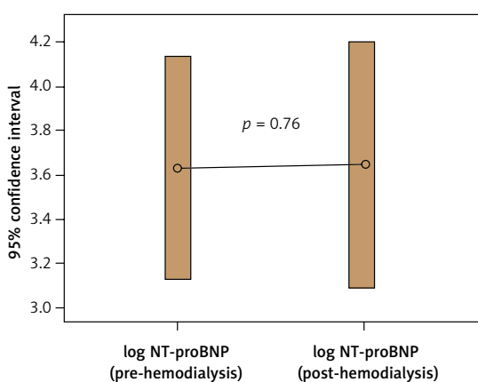
Figure 2. Comparison of the log NT-proBNP levels in pre- and post-hemodialysis patients
