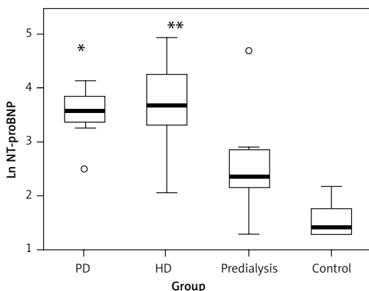
Figure 1. Ln NT-proBNP levels of groups. Ln NT-proBNP level = log N-terminal pro-brain natriuretic peptide
